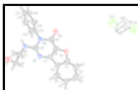
Fig. 1. View of the molecular structure of the title compound, showing the atom labelling scheme and with displacement ellipsoids drawn at 50% probability level. [Symmetry code: (a) - x , y , - z +3/2].
